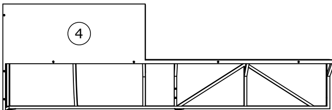
1780x580x90 mm
