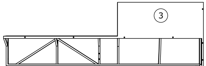
1780x580x90 mm
